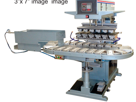
1 Unit 6 Color w/ 22 station conveyor Conveyor mounted flame unit 3"x 7" image image
